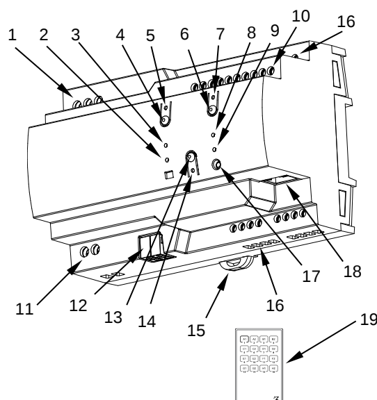
Figure 1: ALLinBOX 88
